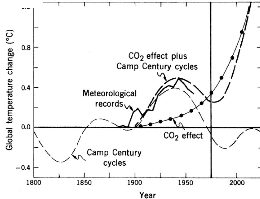
Fig. 1. Curves for the global temperature change due to chemical fuel \text{CO}_2 , natural climatic cycles, and the sum of the two effects. The measured temperature anomaly for successive 5-year means from meteorological records over the last century is given for comparison.
