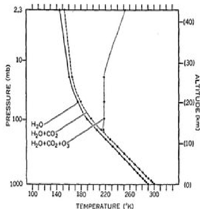
FIG. 6c. Thermal equilibrium of various atmospheres which have a critical lapse rate of 6.5 \text{ deg km}^{-1} . Vertical distributions of gaseous absorbers at 35N, April, were used. S_c = 2 \text{ ly min}^{-1} , \cos \bar{\tau} = 0.5 , r = 0.5 , no clouds.
