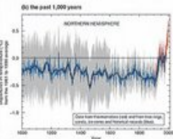
Figure 1: Variations of the Earth's surface temperature over the last 140 years and the last millennium.
