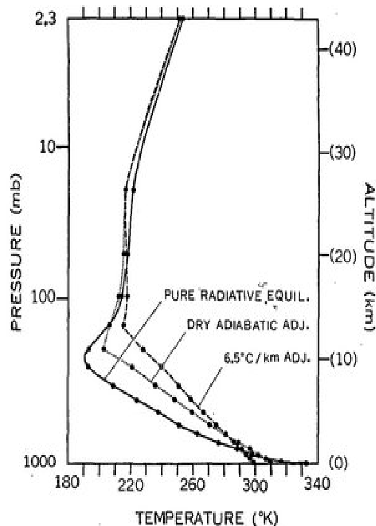
FIG. 4. The dashed, dotted, and solid lines show the thermal equilibrium with a critical lapse rate of 6.5 \text{ deg km}^{-1} , a dry-adiabatic critical lapse rate ( 10 \text{ deg km}^{-1} ), and pure radiative equilibrium.
