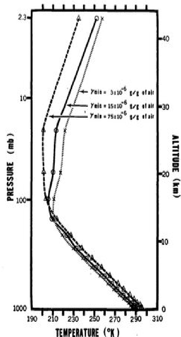
FIG. 12. Vertical distributions of radiative convective equilibrium temperature for various values of water vapor mixing ratio in the stratosphere.
