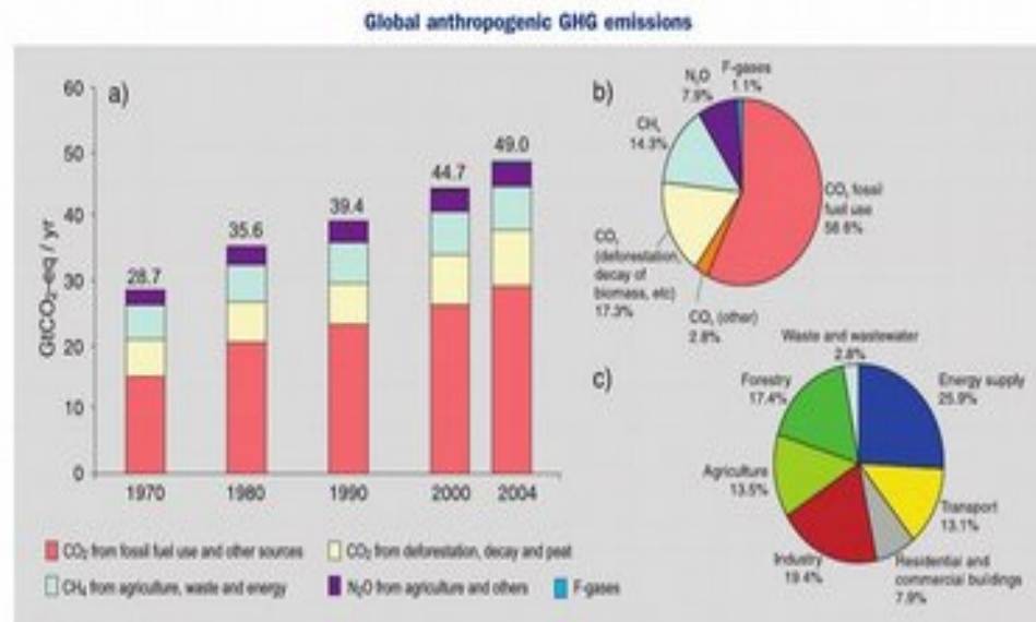
Figure SPM.3. (a) Global annual emissions of anthropogenic GHGs from 1970 to 2004. 1 (b) Share of different anthropogenic GHGs in total emissions in 2004 in terms of carbon dioxide equivalents (CO 2 -eq). (c) Share of different sectors in total anthropogenic GHG emissions in 2004 in terms of CO 2 -eq. (Forestry includes deforestation.) (Figure 2.1)
