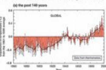
Variations of the Earth's surface temperature for:
