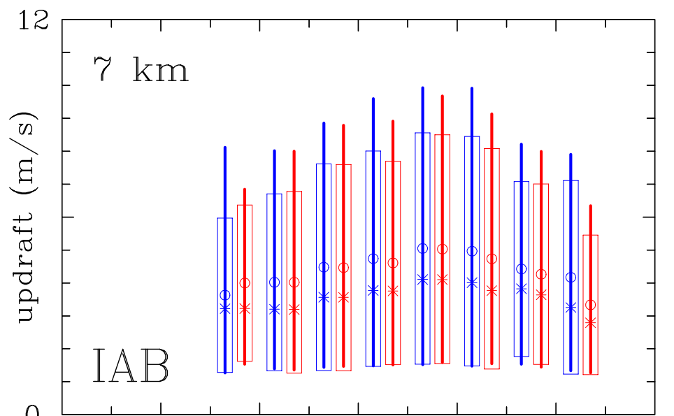
updraft statistics at 3km (10 degC) and 7 km (-12 degC) for w > 1 m/s, q > 1 g/kg
