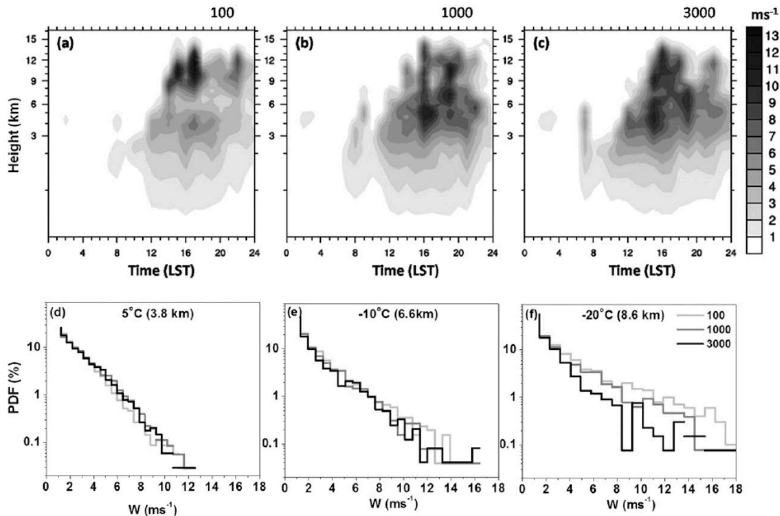
FIG. 11. (top) Time evolution of vertical profiles of simulated maximum updraft in the selected study region for CCN concentrations of (a) 100, (b) 1000, and (c) 3000 \text{cm}^{-3} where updrafts are greater than 1 \text{ m s}^{-1} . (bottom) PDFs (%) over the whole domain at (d) 5^\circ\text{C} , (e) -10^\circ\text{C} , and (f) -20^\circ\text{C} during 1500–1800 LST are also shown.
