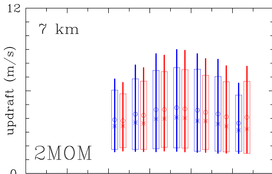
updraft statistics at 3km (10 degC) and 7 km (-12 degC) for w > 1 m/s, q > 1 g/kg
