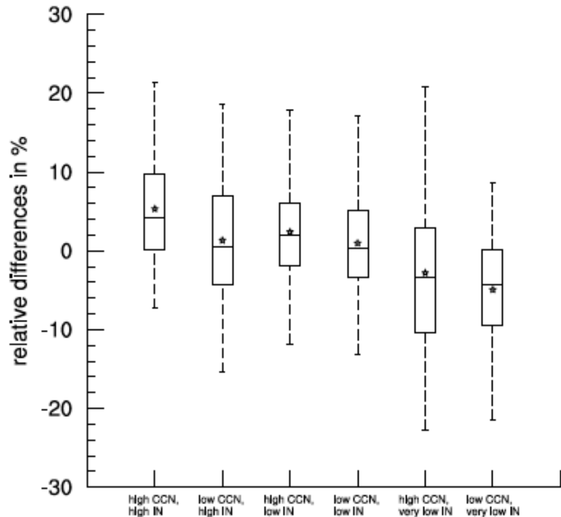
Fig. 9. Box-whisker plot of relative change of 12-h accumulated area-averaged precipitation of JJA 2008–2010. Shown are anomalies relative to the mean of Exps. 1–6. The precipitation data has been averaged over either one of the three subdomains. The bottom and top of the boxes are the lower and upper quartiles, the line near the middle of the boxes is the median, whiskers are the 5th and 95th percentiles and the stars represent the mean value.
