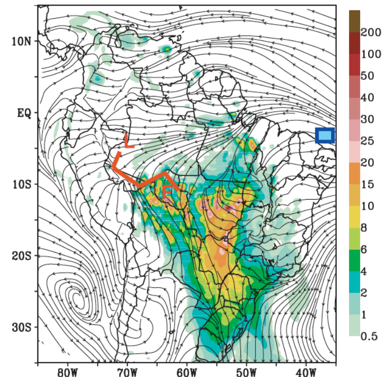
Fig. 1. Smoke aerosol distribution ( D < 2.5 \mu\text{m} ; in \mu\text{g m}^{-2} ) and wind field in the BL over South America during the transect flights from Rondonia to the western Amazon. The aerosol distribution was obtained with the use of the Geostationary Operational Environmental Satellites–Automated Biomass Burning Algorithm (GOES ABBA) Fire product to estimate smoke emissions and the RAMS model to simulate their transport and removal (38). The flight track is indicated as a red line; the study area off Fortaleza, by a blue rectangle; and letters L and F represent the locations of the LET and FNS sounding sites, respectively (fig. S1).
