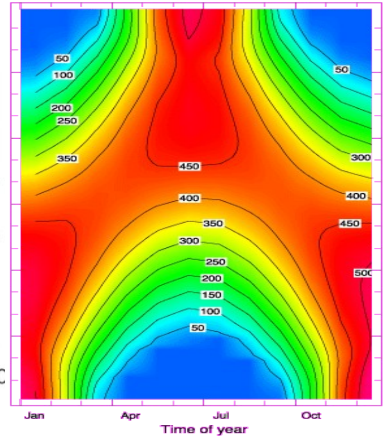
Latitude-Time Distribution of Incoming Solar Radiation at the Top of the Atmosphere
