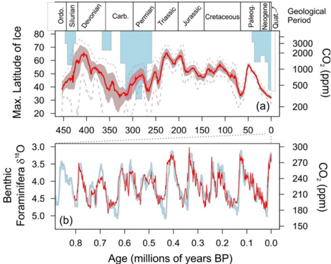
Fig. 1. Carbon dioxide and climate through the Phanerozoic. (a) Latitudinal extent of continental ice deposits shown as blue bars (left axis) and atmospheric CO 2 content (red, right axis). (b) A close-up of the last 0.8 million years comparing CO 2 from ice cores (red, right axis) with benthic foraminiferal oxygen isotope ratios (δ 18 O) (blue, left axis).
