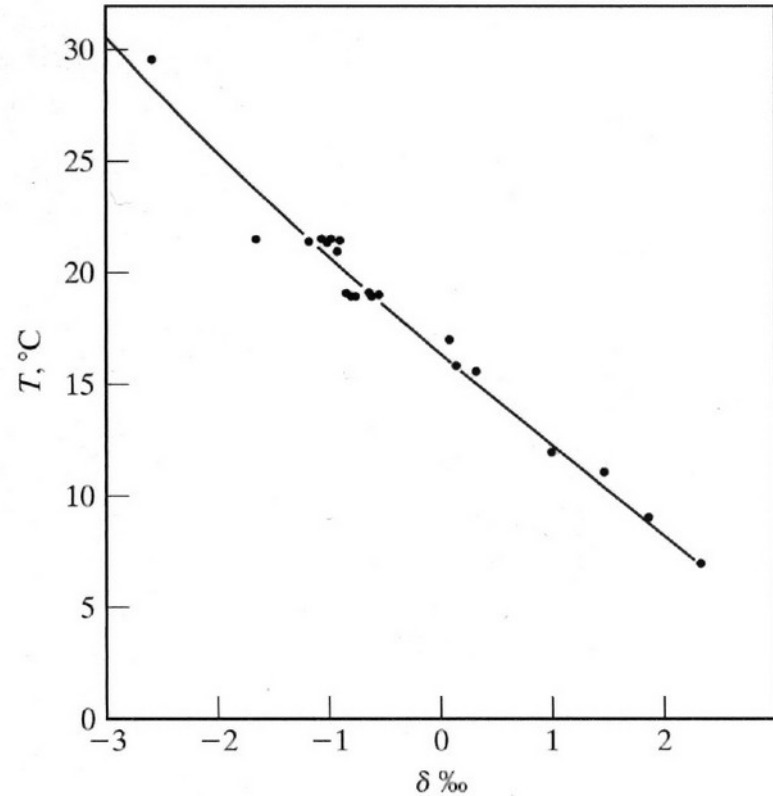
FIGURE 6.2: Plot of Epstein et al.'s (1953) corrected data set for determining the fractionation factor for carbonate–water. The x -axis ( \delta\text{‰} ) refers to the (\delta_{\text{c}} - \delta_{\text{w}}) of equation (6.4), while T(^{\circ}\text{C}) is the measured water temperature. Reprinted with permission from the Geological Society of America.
