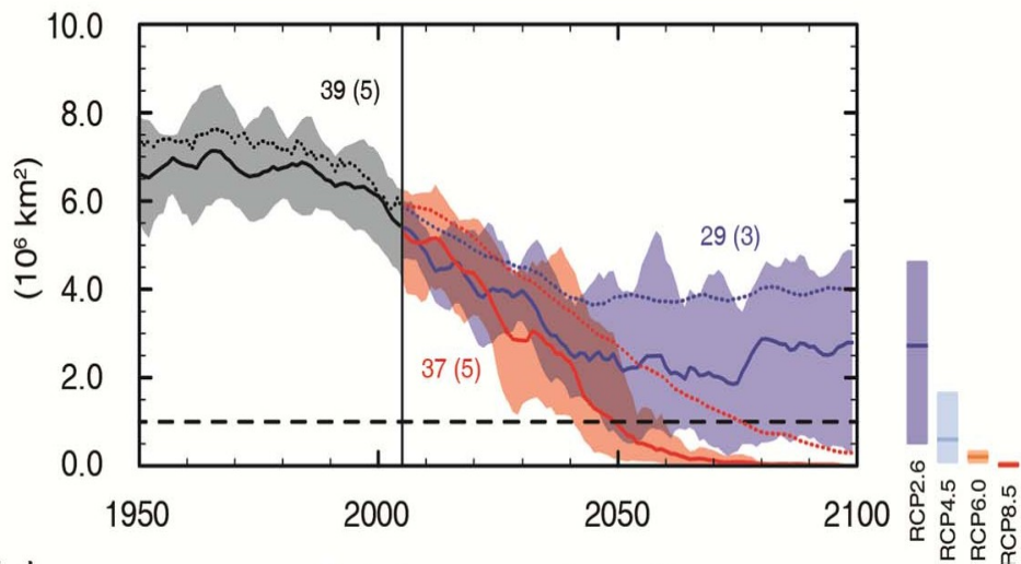
(b) Northern Hemisphere September sea ice extent
