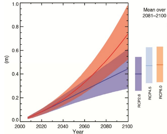
Global mean sea level rise
